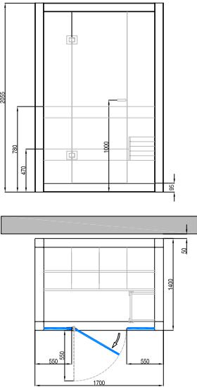
Porta reversibile Reversible door
