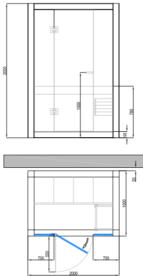
Porta reversibile Reversible door
